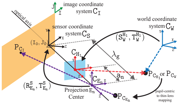
Figure 3. Coordinate Systems for non-frontal camera calibration.
